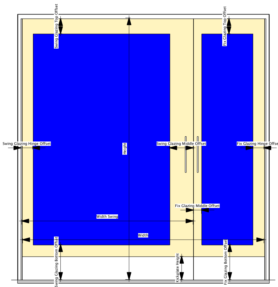
ELEVATION DIMENSIONS DOUBLE DOORS & GLAZING OPENING
