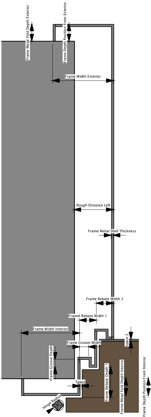
PLAN DETAIL OF METAL FRAME TYPE 1
